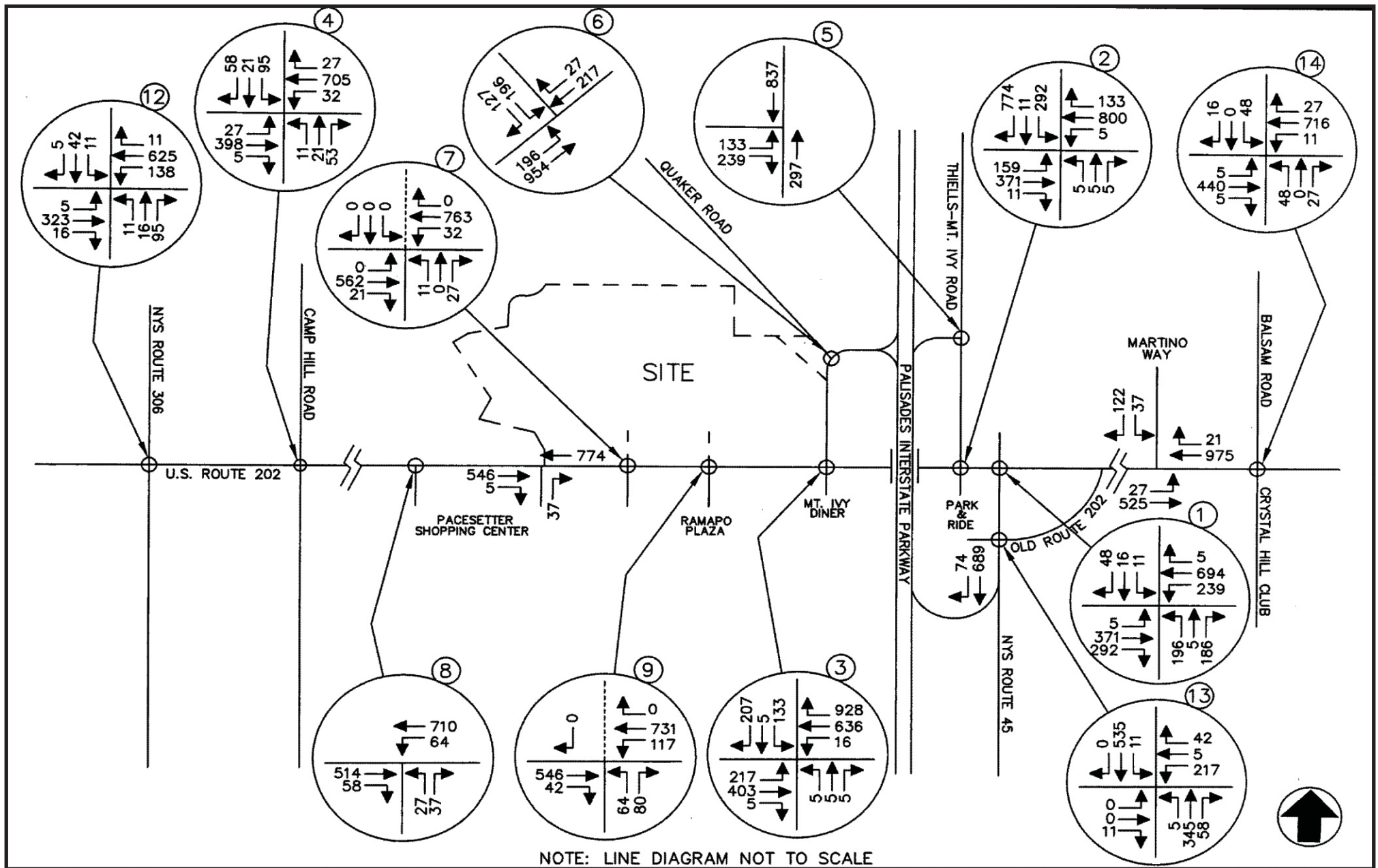
Figure 3.5-5: 2011 Projected Traffic Volumes Weekday Peak AM Highway Hour Minisceongo Park
